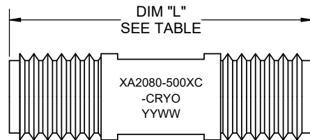
ADAPTER, SMA-f/f, DC-18 GHz, CRYO
