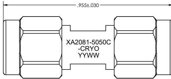
ADAPTER, SMA-m/f, DC-18GHz, CRYO
