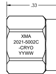
SMA-m, OPEN, CRYO
