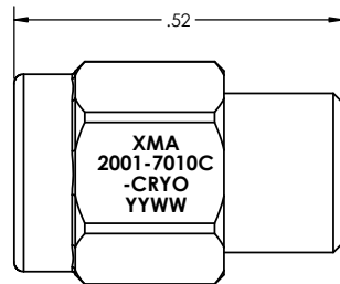
TERMINATION, SMA-m, DC-18GHz, 2W, CRYO
